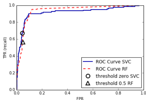
Figure 5-16. Comparing ROC curves for SVM and random forest
