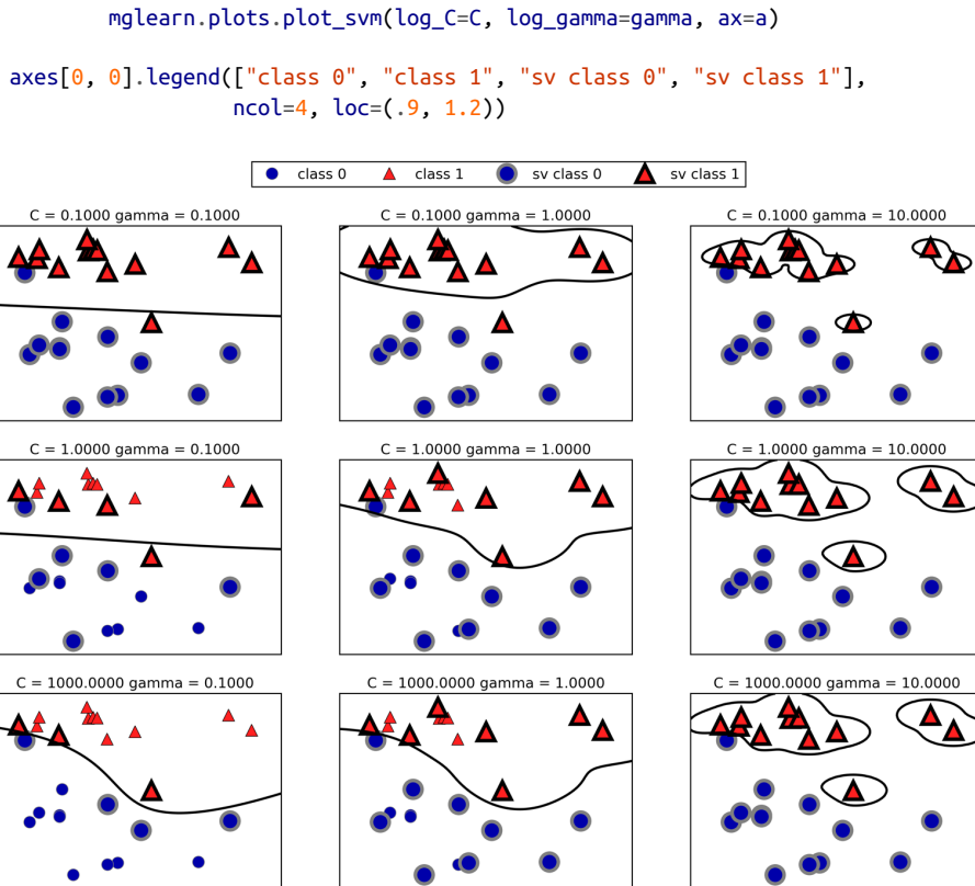
Figure 2-42. Decision boundaries and support vectors for different settings of the parameters C and \gamma
