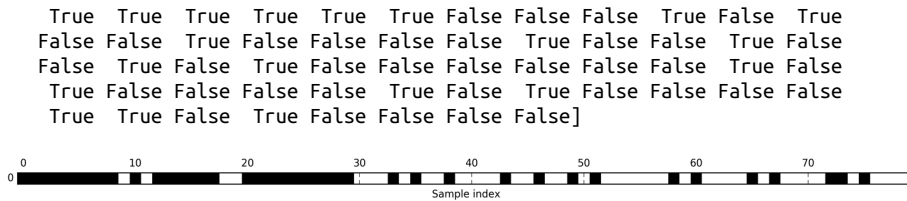
Figure 4-9. Features selected by SelectPercentile
