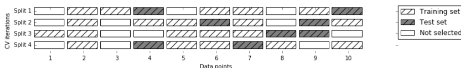
Figure 5-3. ShuffleSplit with 10 points, train_size=5 , test_size=2 , and n_splits=4
