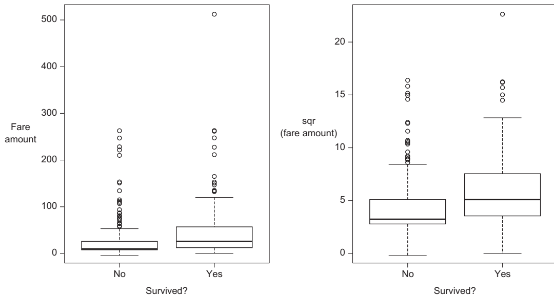
Figure 2.15 Box plots showing the relationship between passenger fare paid and survival on the Titanic. The square-root transformation makes it obvious that passengers who survived paid higher fares, on average.
