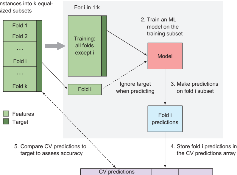
Figure 4.7 Flowchart of k -fold cross-validation
