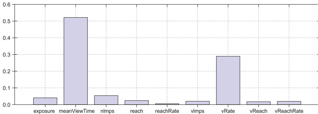
Figure 10.7 Variable importance for the random forest regression
